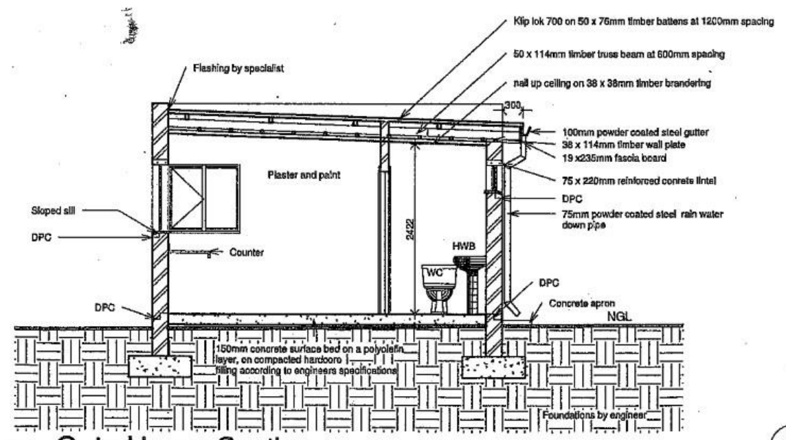
6 Gate House Section 1 : 50
