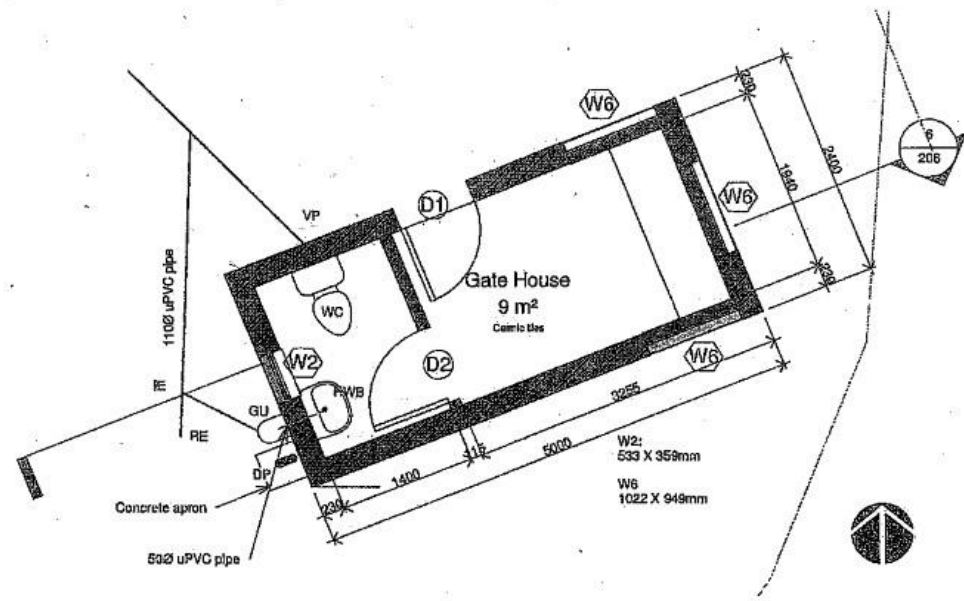
1 Gate House 1 : 50
