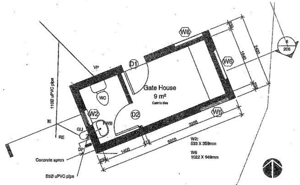
1 Gate House 1 : 50
