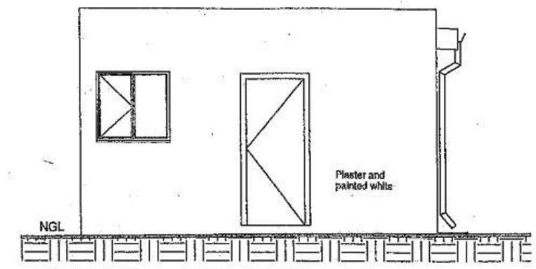
2 Gate House North Elevation 1 : 50
