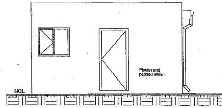
2 Gate House North Elevation 1 : 50
