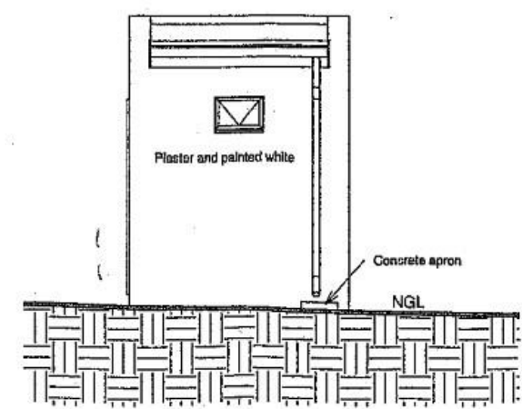
5 Gate House West Elevation 1 : 50
