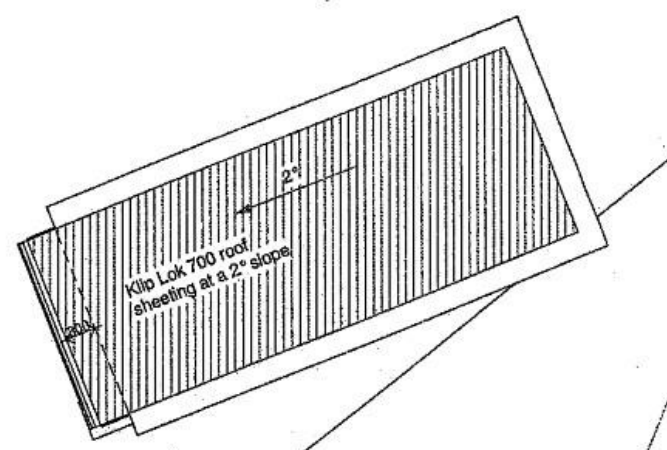
7 Gate House Roof plan 1 : 50
