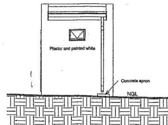
5 Gate House West Elevation 1 : 50
