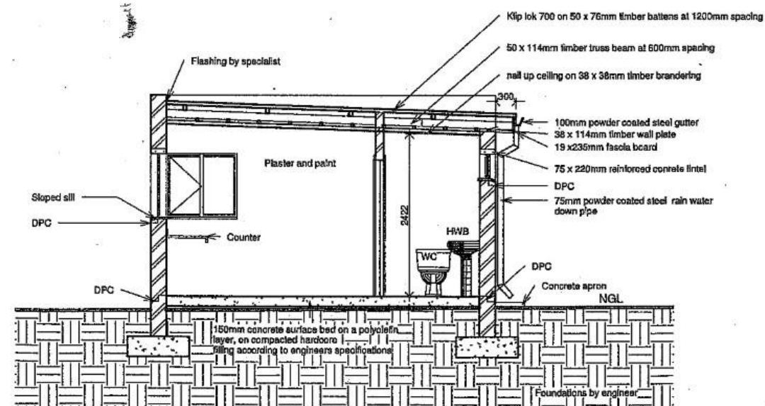
6 Gate House Section 1 : 50
