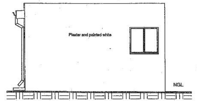
3 Gate House South Elevation 1 : 50
